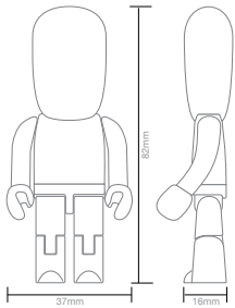
original USM6092
